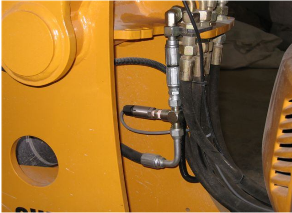
Typical Installation of the ED2 Series Pressure Transducer in Lifting Hydraulic Circuit
